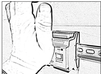
Fig. 4: Pressing the device onto the profile rail
