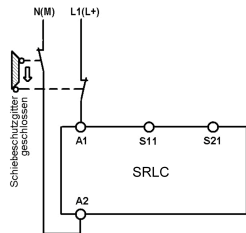
Fig. 3: Two-channel sliding guard monitoring with positively driven limit switches. (up to category 3, PL d)
