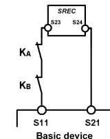
Fig. 4: Feedback Loop with Auto-Start
