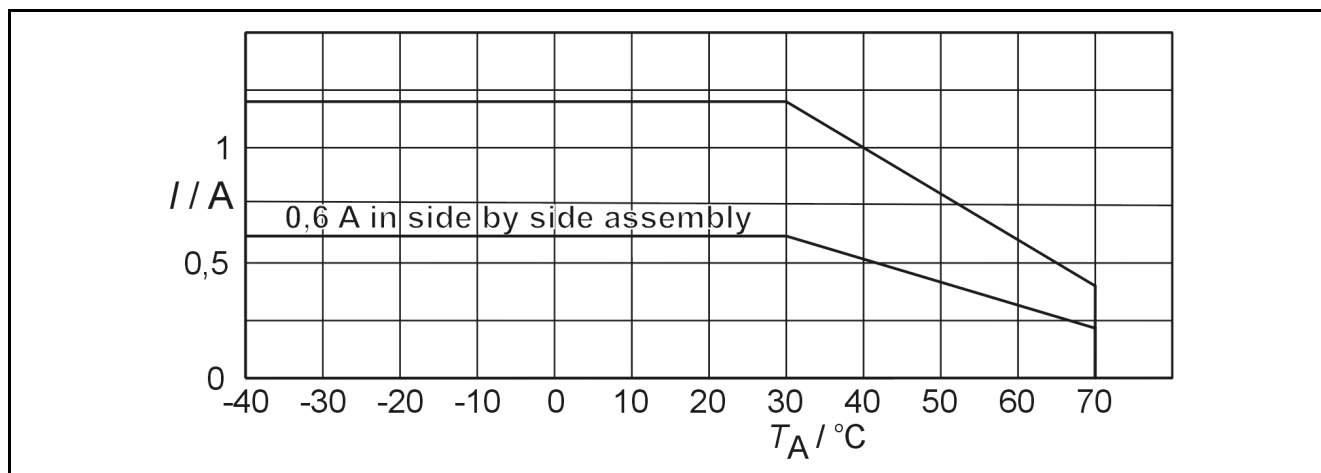
Derating curve for SLO 5IRA.
