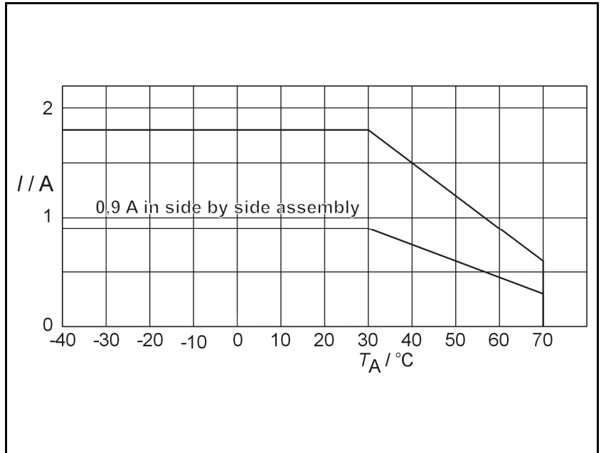
Derating curve for SLO 48CRA.
