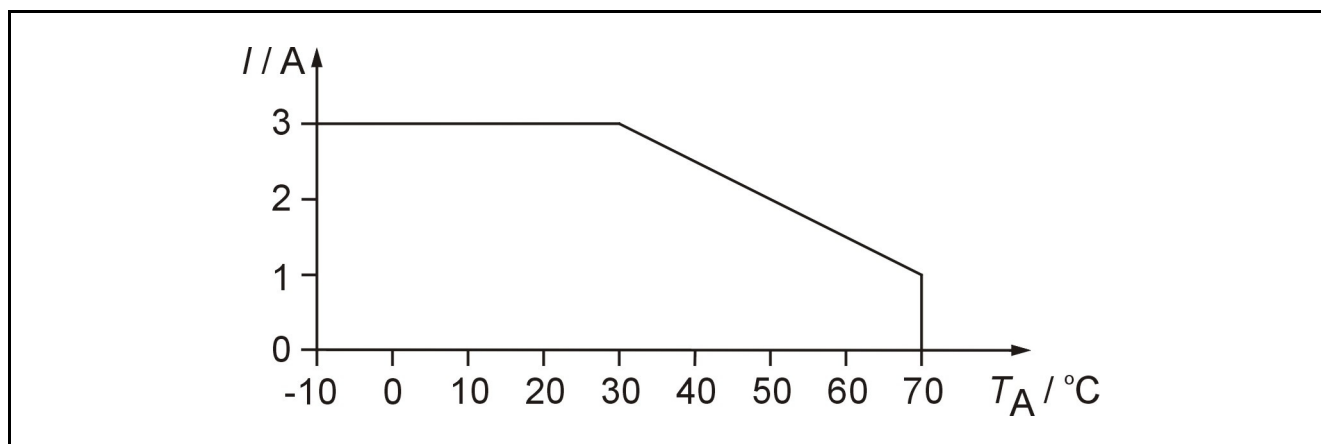
Derating curve for SLO 24TR.
