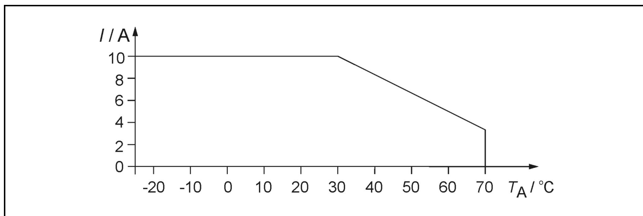
Derating curve for SLO 24CRXSN.
