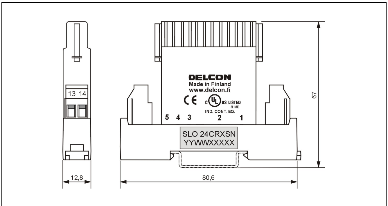
SLO 24CRXSN (dimensions in mm).
