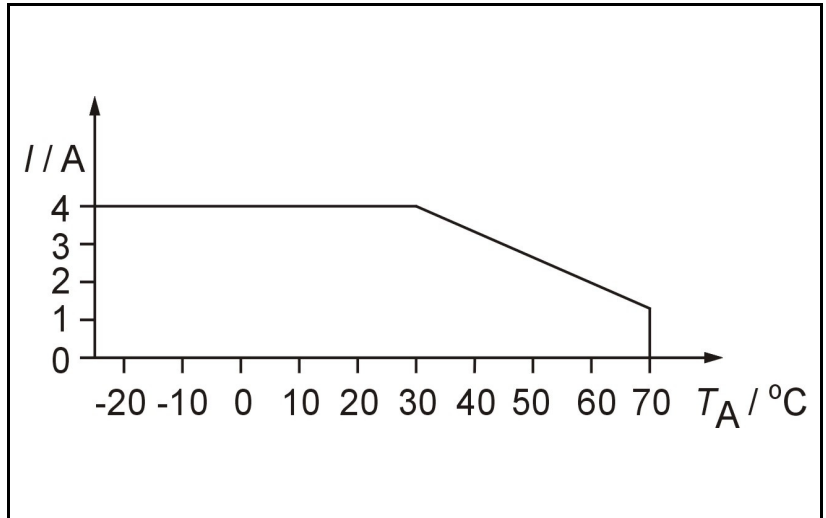
Derating curve for SLO 24CRA4.
