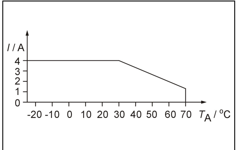
Derating curve for SLO 220CRA4.
