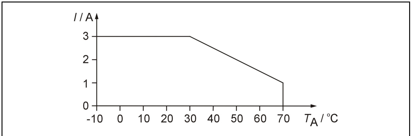
Derating curve for SLO 12TR.
