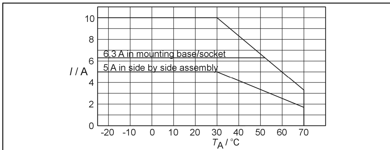
Derating curve for SLO 12CRX.
