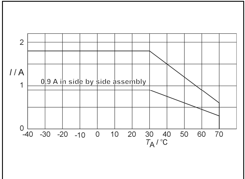
Derating curve for SLO 12CRA.
