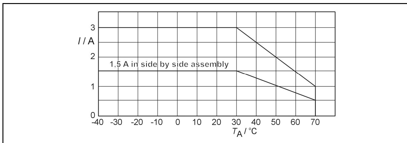
Derating curve for SLO 12CR.
