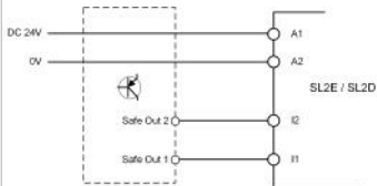
Fig. 13 OSSD outputs dual channel
