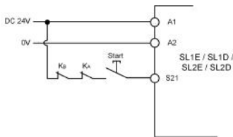
Fig. 16 Manual start with feedback circuit
