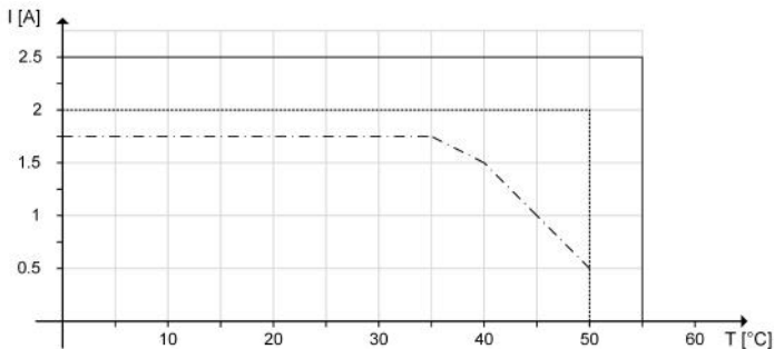
Fig. 26 Derating curve
