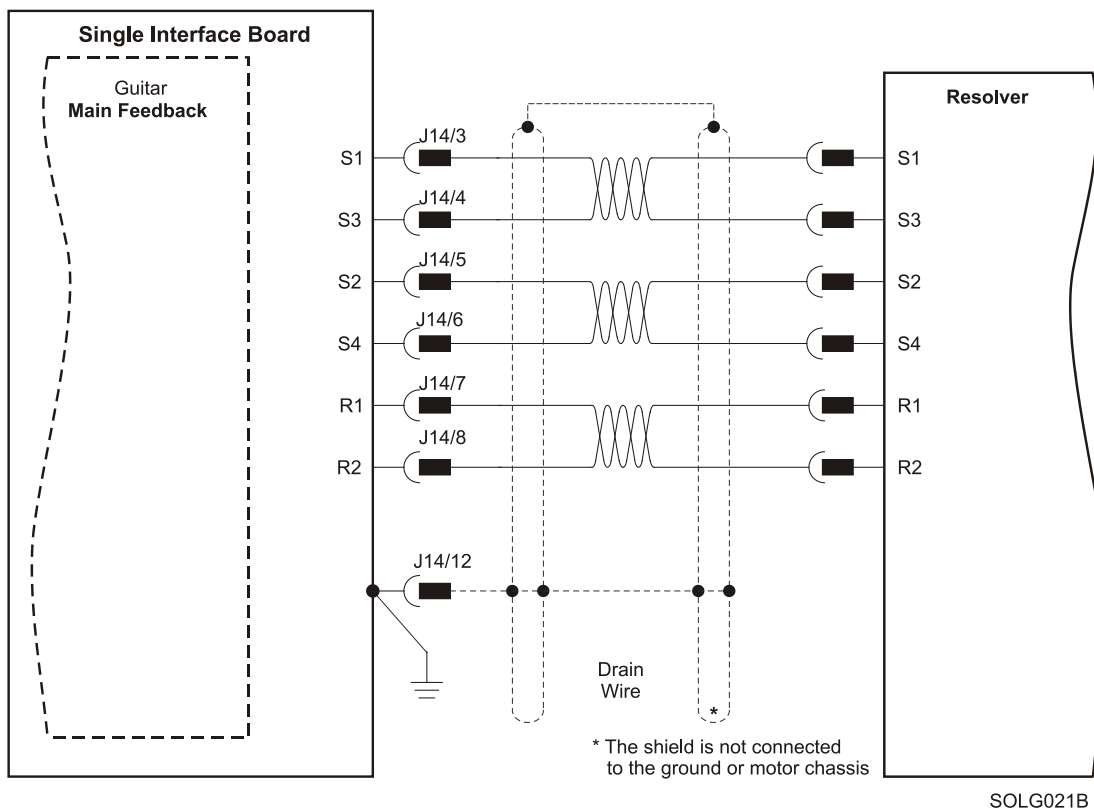
Figure 10: Main Feedback – Resolver Connection Diagram
