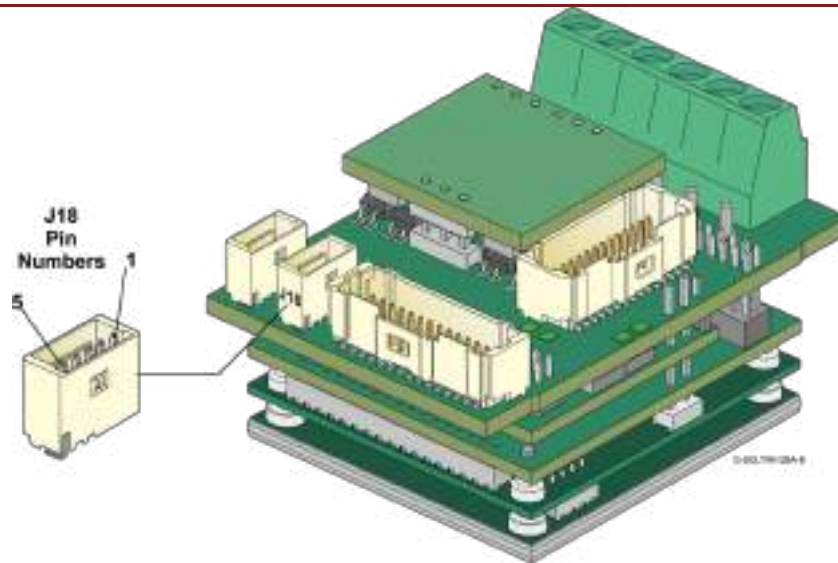
EtherCAT OUT Pin Assignments
