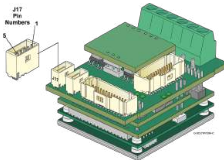
EtherCAT IN / Ethernet Pin Assignments
