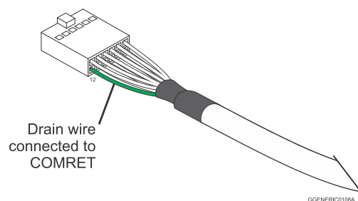
Figure 4: Feedback and Molex Control Cable Assemblies
