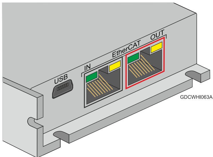
8-Pin RJ-45
