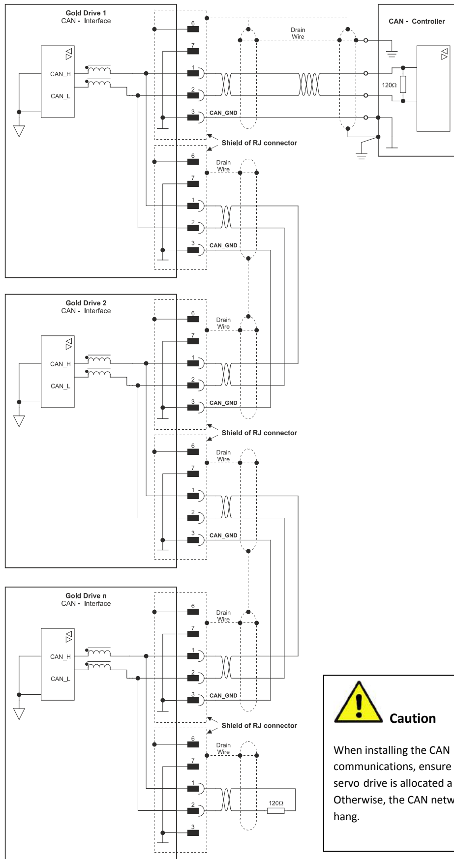
Figure 40: Gold DC Whistle Connection Diagram – CAN
