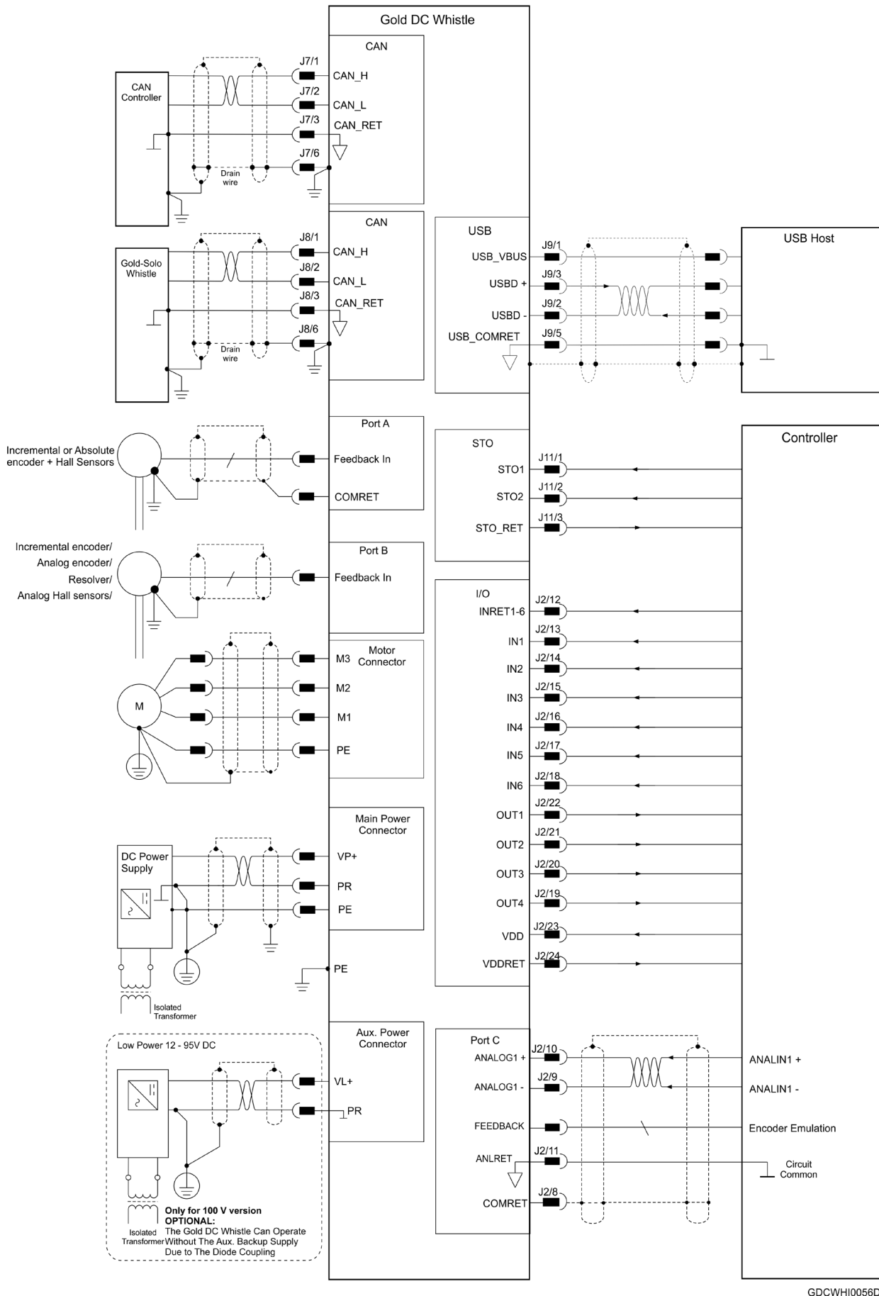
Figure 3: The Gold DC Whistle Connection Diagram - CAN
