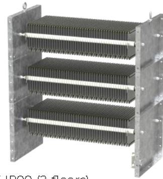
LAGC-LV IP00 (3 floors)
