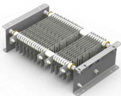
Laser Cut Grid (350 x 190mm)
