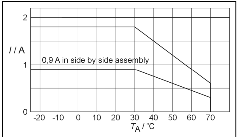
Derating curve for EXO 5CHA.
