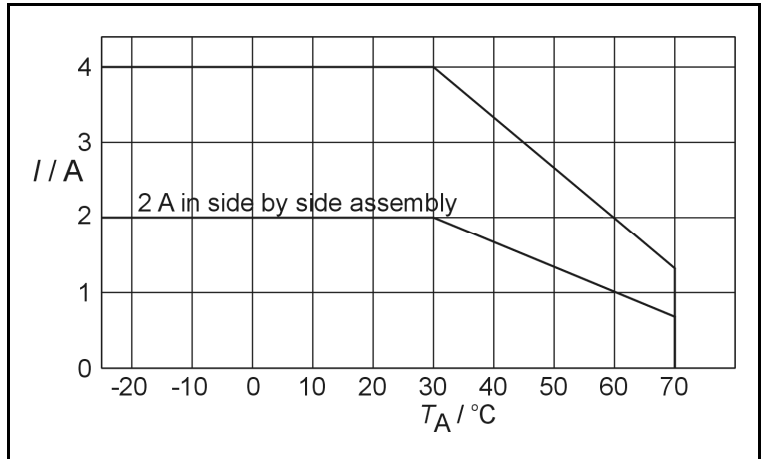
Derating curve for EXO 48CHA4.
