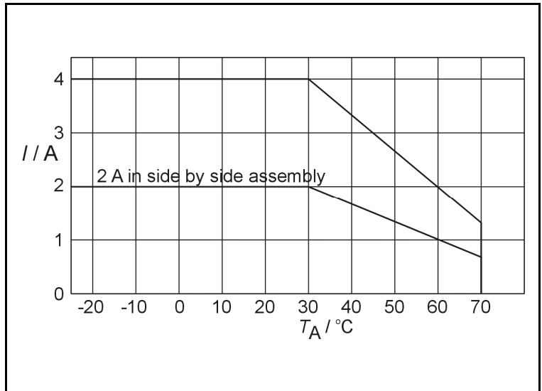
Derating curve for EXO 24CHA4.
