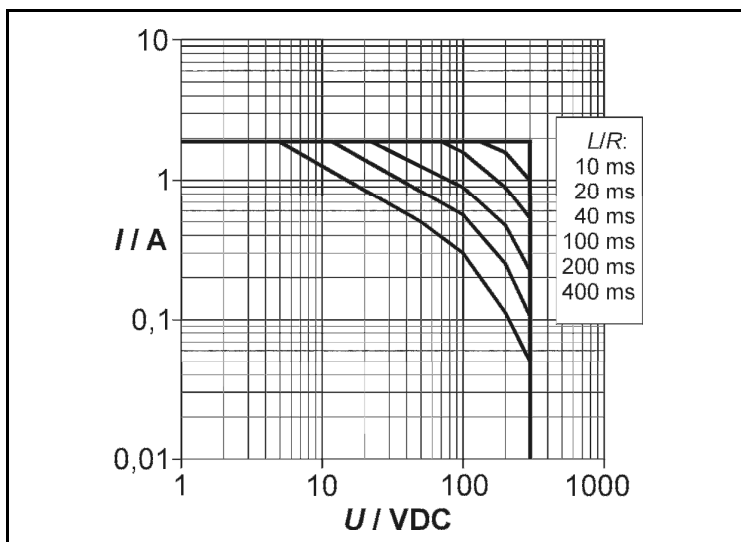
Derating curve for inductive loads.
