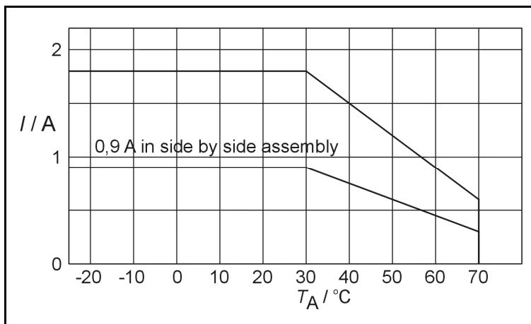
Derating curve for EXO 24CHA.
