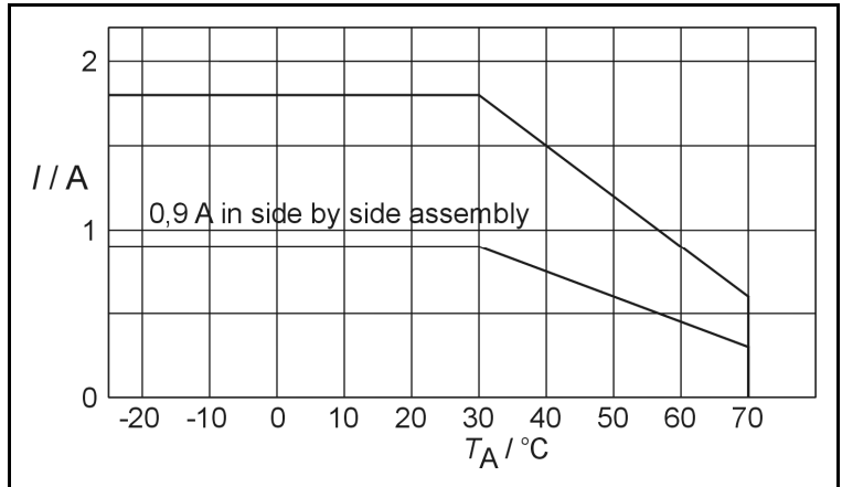
Derating curve for EXO 12CHA.
